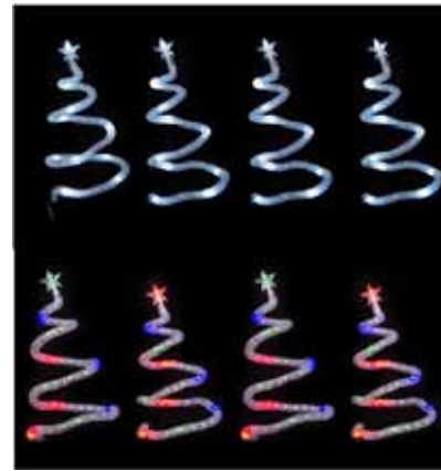
-779- XA8899 CTN: 12 SOLAR MESH SPIRAL TREE 4PC M/W SIZE: Height: 37cm NOTES: Solar Panel 2V 80mA. 1 x AA 1.2V 600mAh NI-MH Battery. 1m Green Lead Wire with 100cm LED Spacing Between Trees. 2 Functions: Flashing + Steady. 10 LEDs Each Tree and 40 LEDs in Total
